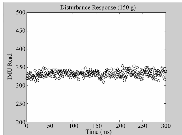
Figure 11. Roll axis hover test response for 150 g load.
