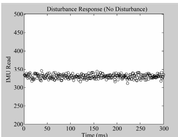
Figure 15. Pitch axis hover test response for no load.
