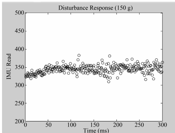
Figure 17. Pitch axis hover test response for 150 g load.
