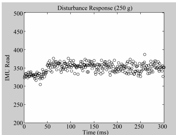
Figure 19. Pitch axis hover test response for 250 g load.
