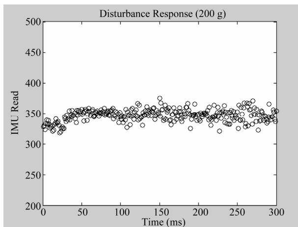
Figure 18. Pitch axis hover test response for 200 g load.
