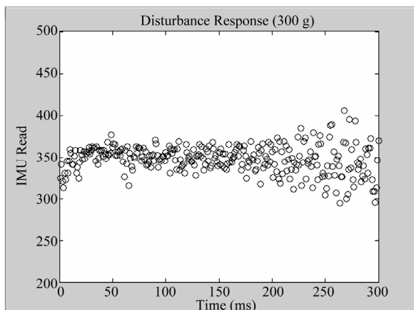
Figure 14. Roll axis hover test response for 300 g load.
