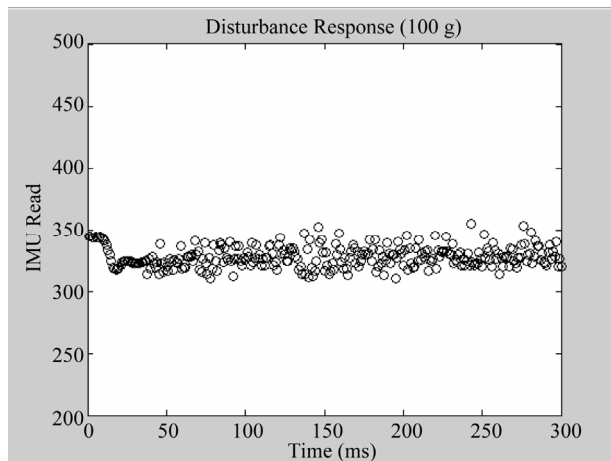
Figure 10. Roll axis hover test response for load 100 g load.
