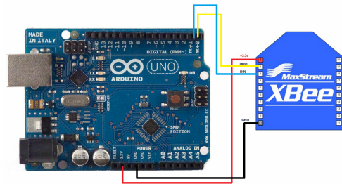
Figure 7. Xbee and Arduino Uno connection.
