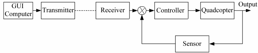
Figure 5. Quadcopter controller.
