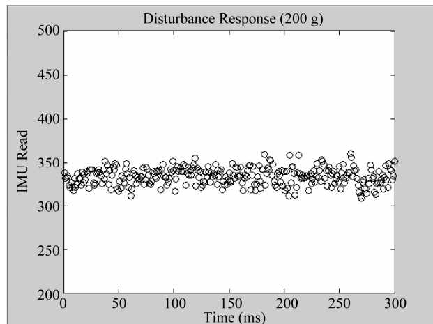
Figure 12. Roll axis hover test response for 200 g load.
