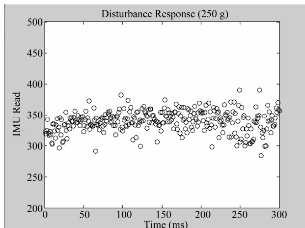
Figure 13. Roll axis hover test response for 250 g load.
