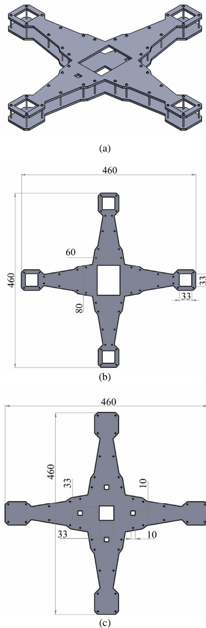
Figure 2. (a) Quadcopter frame; (b) Top view; (c) Botom view.
