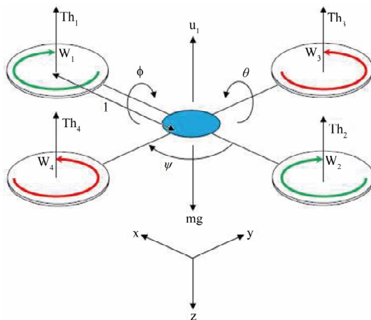
Figure 1. Schematic of Quadcopter.
