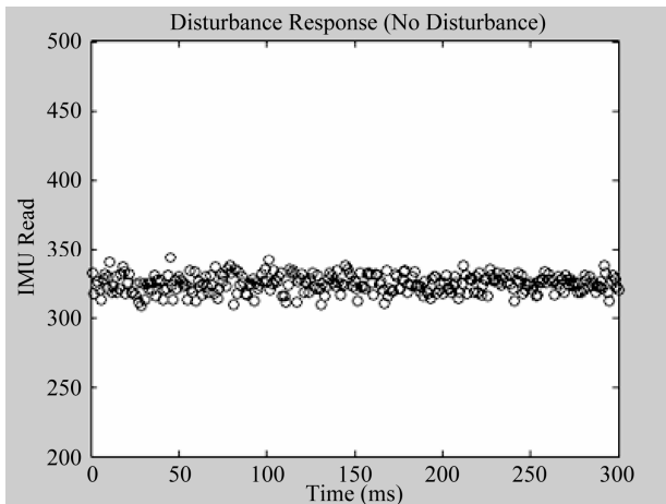
Figure 9. Roll axis hover test response for no load.
