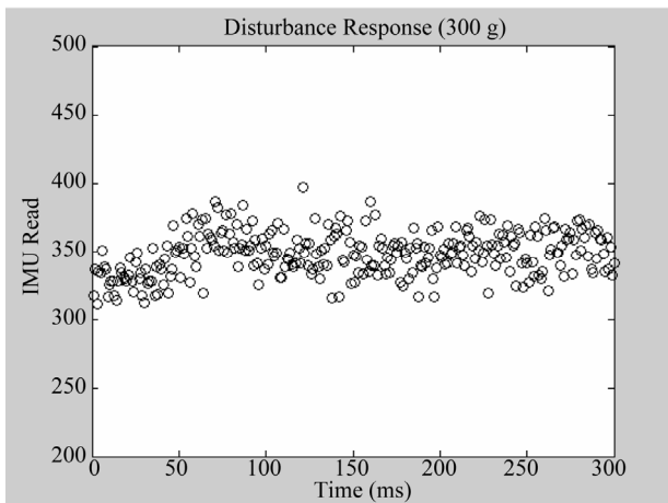
Figure 20. Pitch axis hover test response for 300 g load.
