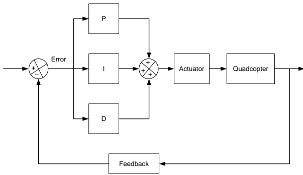
Figure 8. Block of Quadcopter PID controller.
